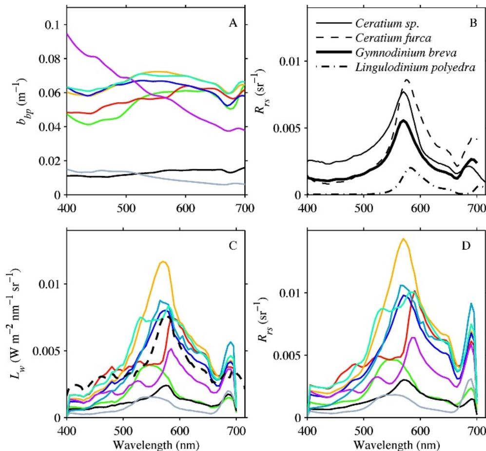
Fig. 2. (A) Backscattering estimated for phytoplankton concentrations of 30 \text{ mg Chl } a \text{ m}^{-3} for each taxon (Stramski et al. 2001), as defined in Fig. 1. (B) Remote sensing reflectance, R_{rs} , measured from a variety of dinoflagellate red tides along the California coast. Lingulodinium polyedra spectrum provided courtesy of G. Chang. (C) Water-leaving radiance, L_w , modeled for dense phytoplankton bloom conditions ( 30 \text{ mg Chl } a \text{ m}^{-3} ) from a variety of phytoplankton taxa. (D) Data from panel (C) shown as R_{rs} .
